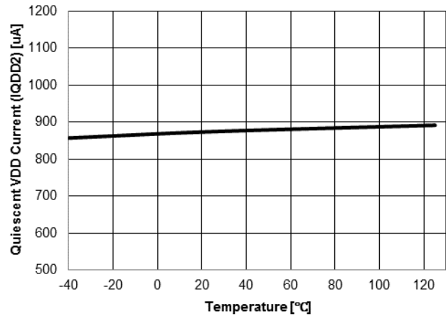
Figure 11. Quiescent Current 2 ( I_{QDD2} ) vs. Temperature
