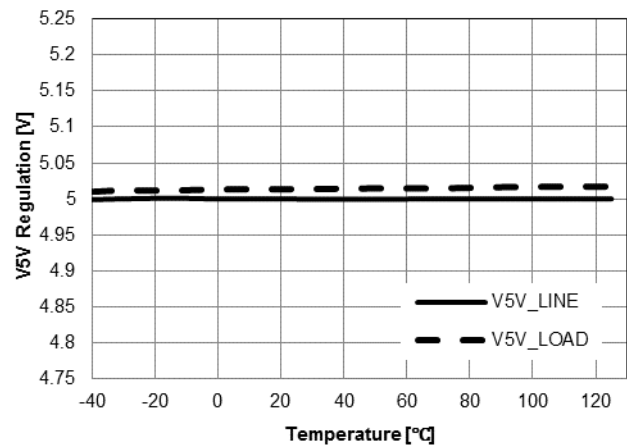
Figure 15. 5 V Regulated Output Voltage (V5V) vs. Temperature
