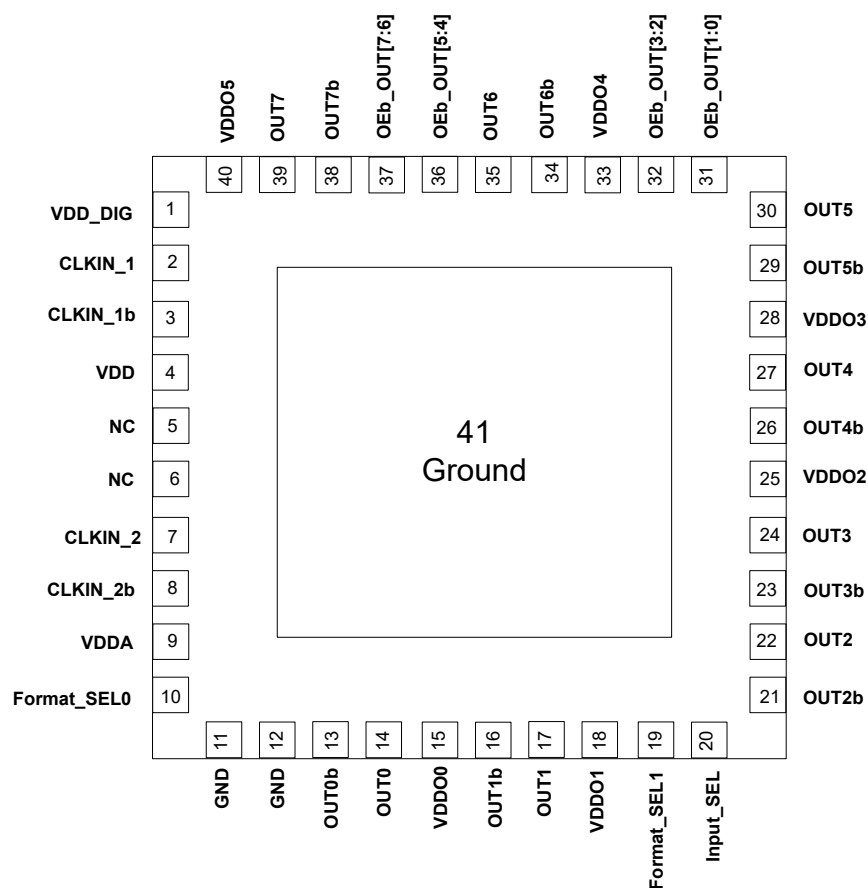
Figure 6.1. Si53358A-D01AM 40-QFN
