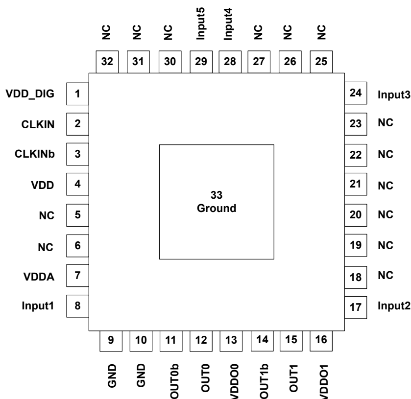
Figure 6.6. Si53352A-Dxxxxx-AM 32-QFN
