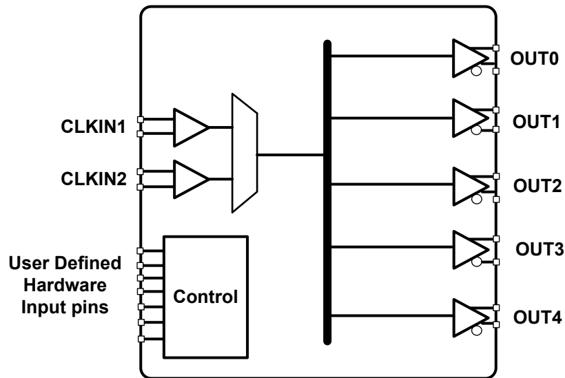
Figure 3.5. Si53354BDxxxxx-AM Functional Block Diagram
