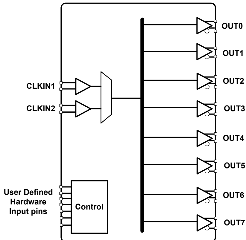
Figure 3.6. Si53358BDxxxxx-AM Functional Block Diagram
