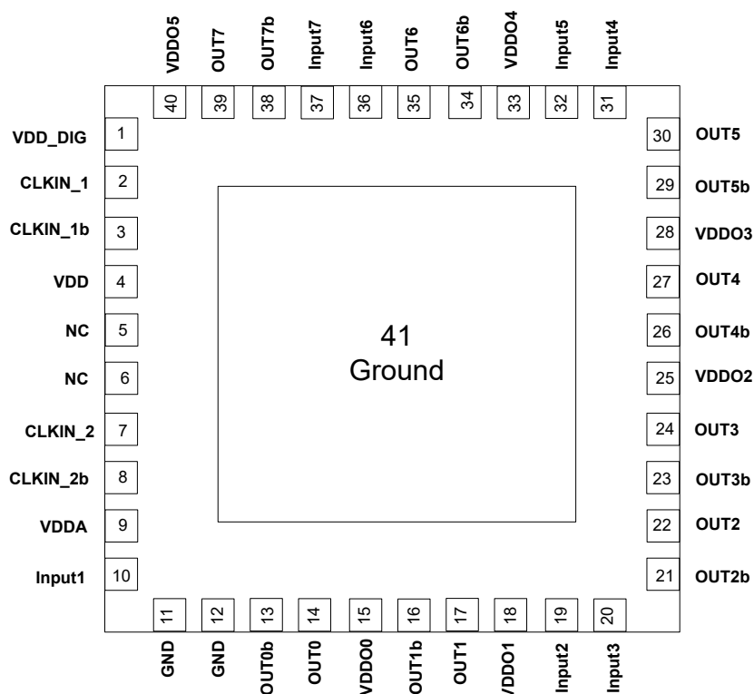
Figure 6.2. Si53358Bxxxxx-AM 40-QFN
