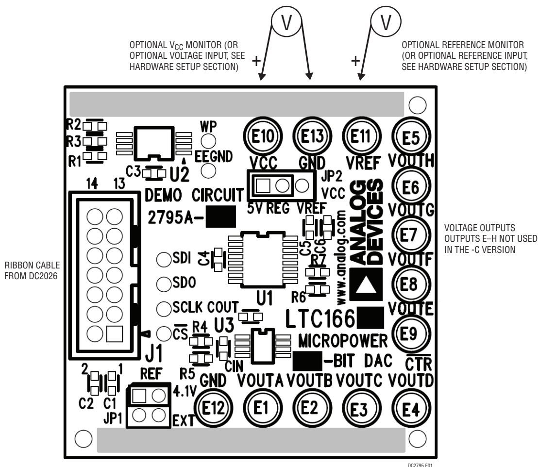
Figure 1. Connection Diagram
