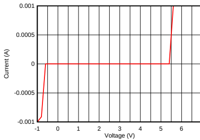
Figure 5. DC Voltage Sweep I-V Curve, I/O Pin to GND
