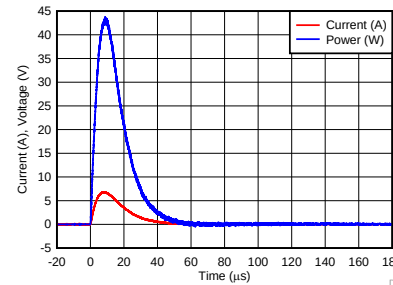
Figure 6. Surge Curve (IEC 61000-4-5, t_p=8/20 \mu s), I/O Pin to GND
