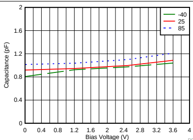
Figure 7. Capacitance vs. Bias Voltage For Different Temperatures ( ^{\circ} C)
