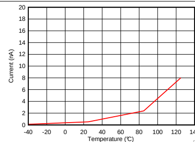
Figure 8. Leakage Current (at 3.6 V Bias) Across Temperature, I/O Pin to GND
