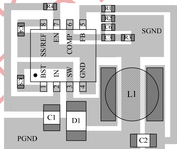
Figure2—PCB Layout
