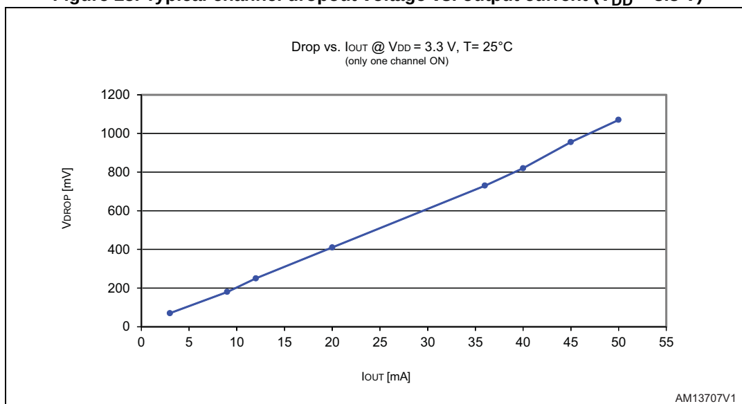
Figure 25. Typical channel dropout voltage vs. output current ( V_{\text{DD}} = 3.3 \text{ V} )
