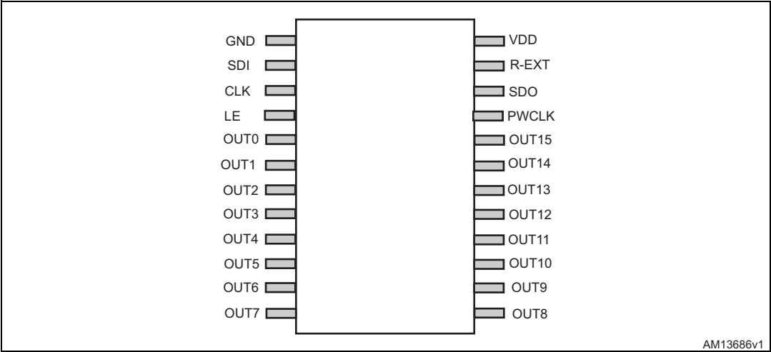
Figure 1. TSSOP24EP pinout
