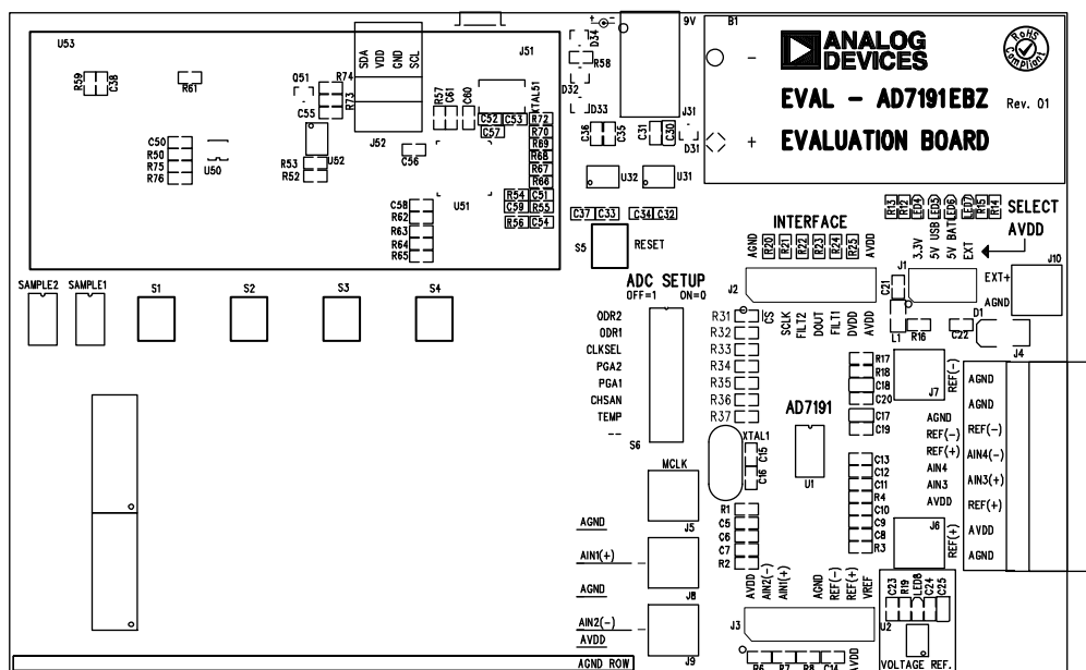
Figure 17. EVAL-AD7191EBZ Silkscreen
