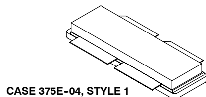
CASE 375D-05, STYLE 1 NI-1230 MRF6VP3450HR6(HR5)
