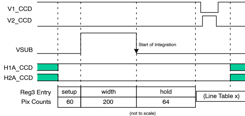
Figure 19. Electronic Shutter Timing
