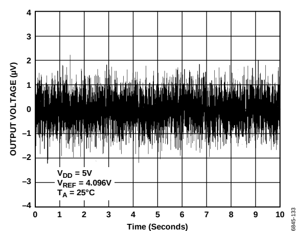
Figure 33. 1/f Noise
