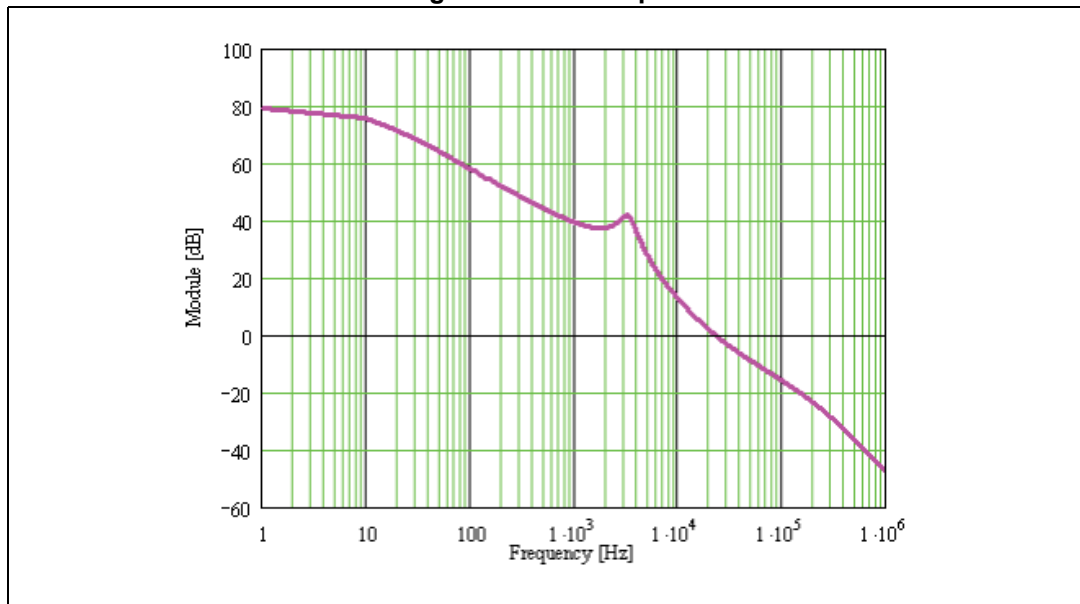
Figure 11. Module plot
