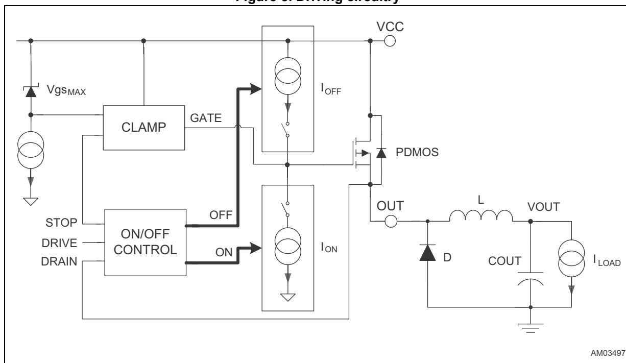
Figure 8. Driving circuitry
