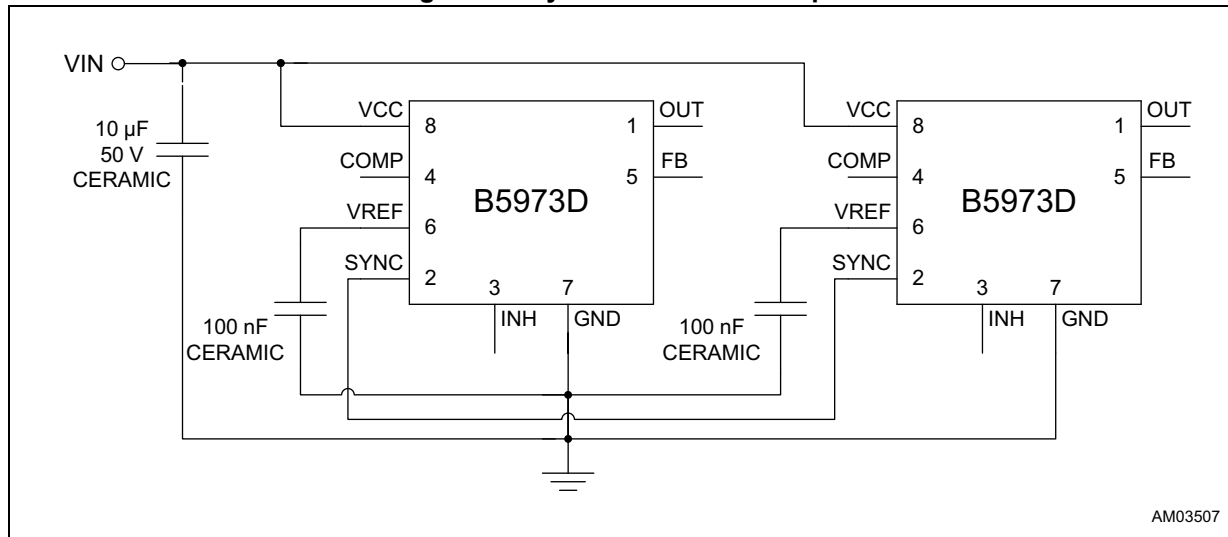
Figure 24. Synchronization example
