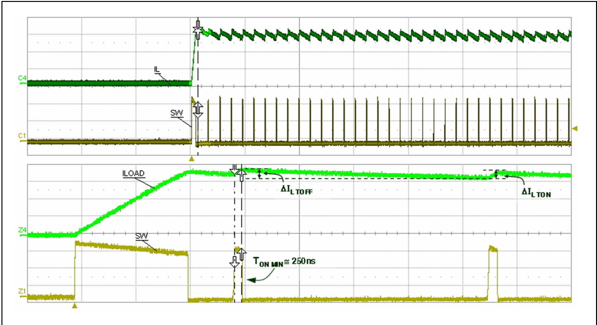
Figure 15. Short-circuit current V_{IN} = 12\text{ V}
