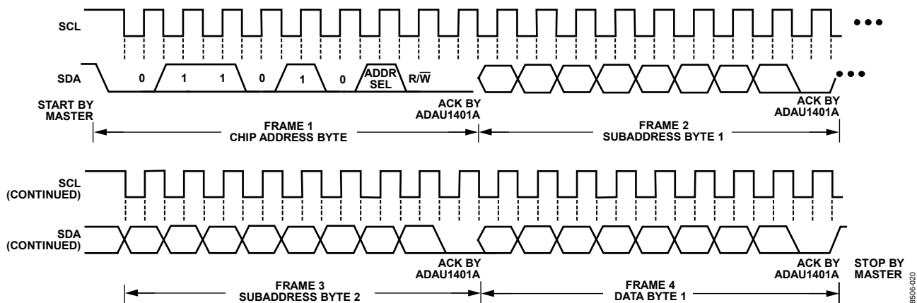
Figure 20. I 2 C Write to ADAU1401A Clocking
