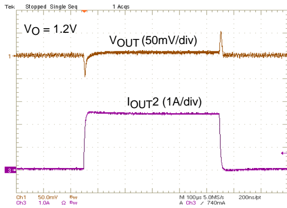
100 μs/div Figure 14. VOUT2 = 1.2V, 0A to 2.5A Load Transient Response
