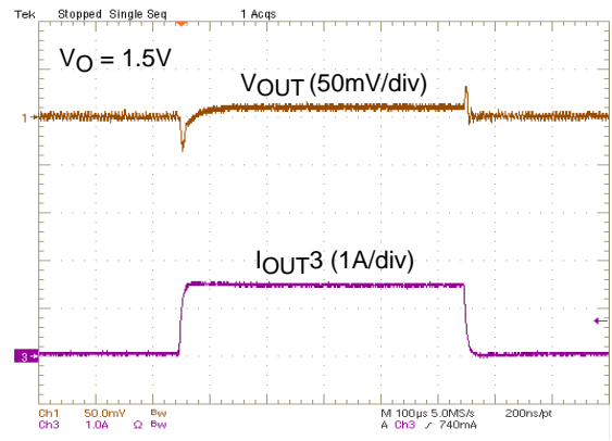
100 μs/div Figure 15. VOUT3 = 1.5V, 0A to 1.5A Load Transient Response
