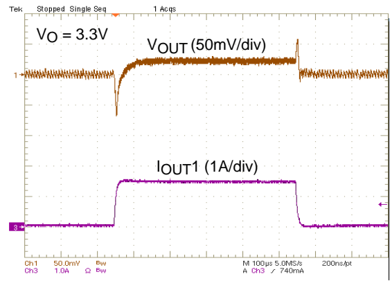
100 μs/div Figure 13. VOUT1 = 3.3V, 0A to 1.5A Load Transient Response
