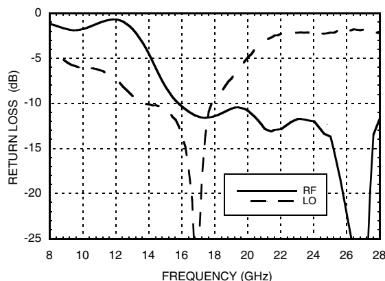
Return Loss
