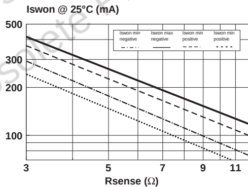
Fig. 30 : Variation of switching-on current versus R_{SENSE} at 25^\circ C .
