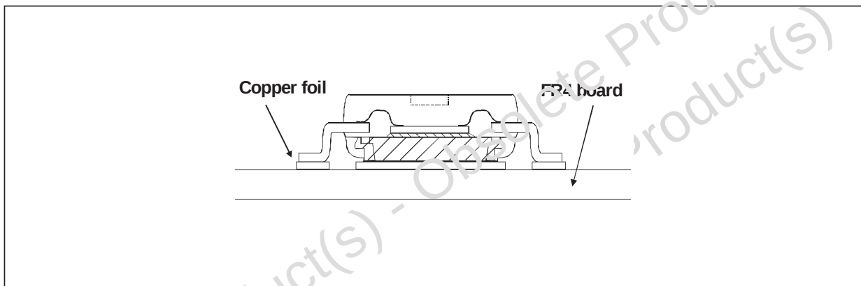
Fig 2 : Mounting on epoxy FR4 heat dissipation by extending the area of the copper layer
