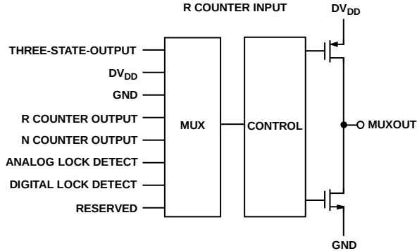
Figure 17. MUXOUT Schematic
