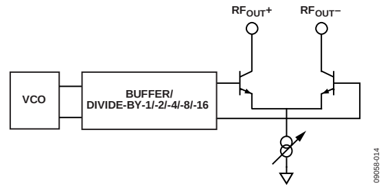
Figure 18. Output Stage
