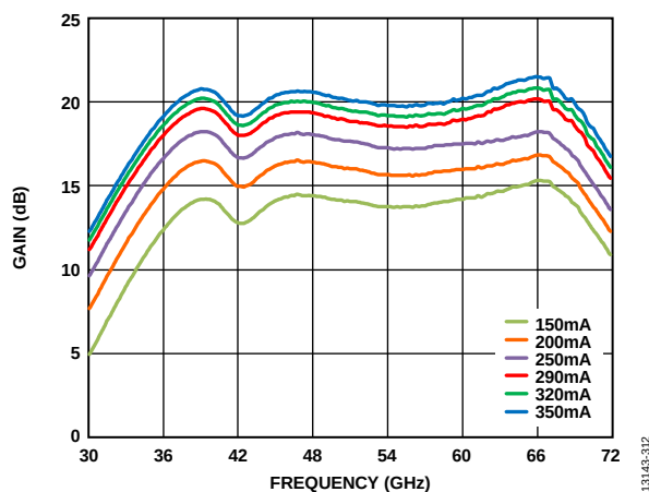
Figure 12. Gain vs. Frequency for Various I_{DD} at V_{DD} = 4 V
