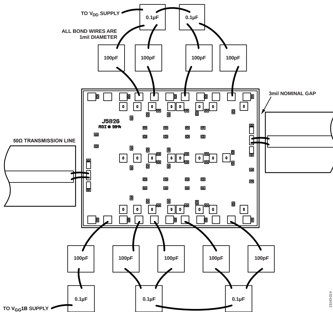
Figure 40. Assembly Diagram
