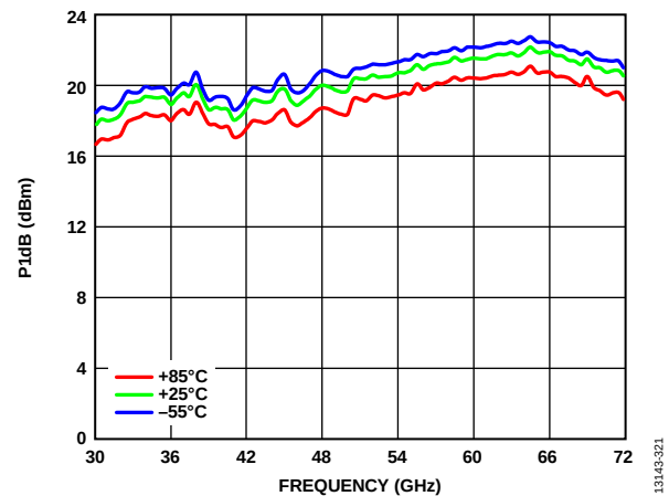
Figure 21. P_{1dB} vs. Frequency at Various Temperatures
