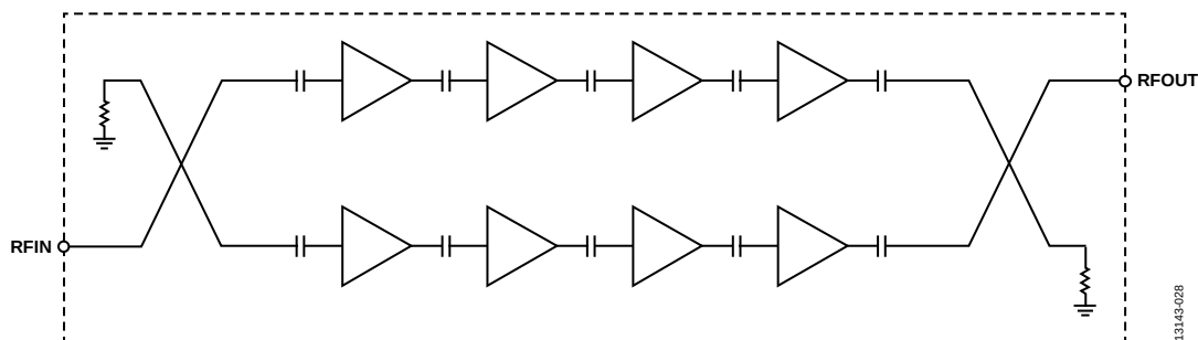
Figure 34. HMC1144 Architecture
