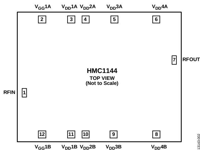
Figure 2. Pad Configuration
