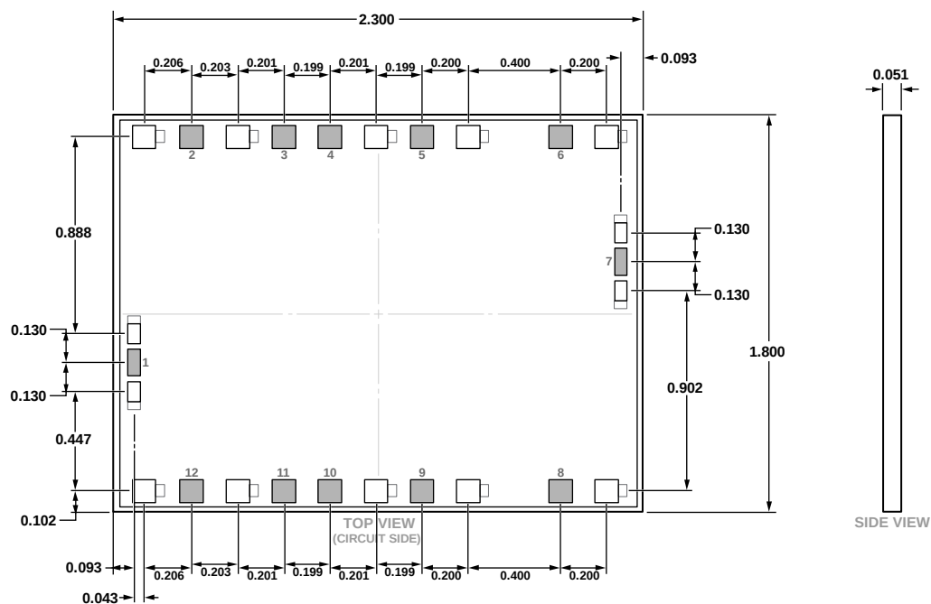
Figure 41. 12-Pad Bare Die [CHIP] (C-12-2)
