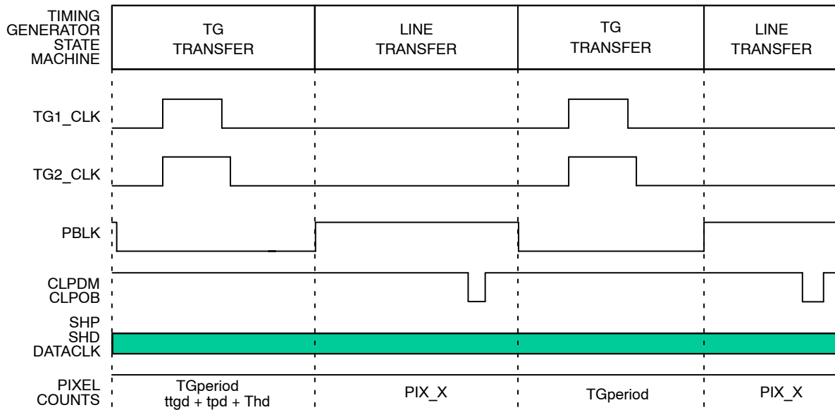
Figure 10. AD9845 Timing
