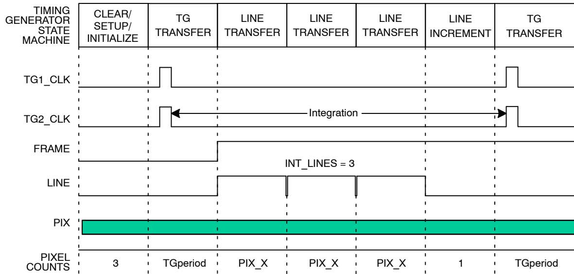
Figure 9. PCI-1424 Frame Grabber Timing – Multi-Line Integration Mode
