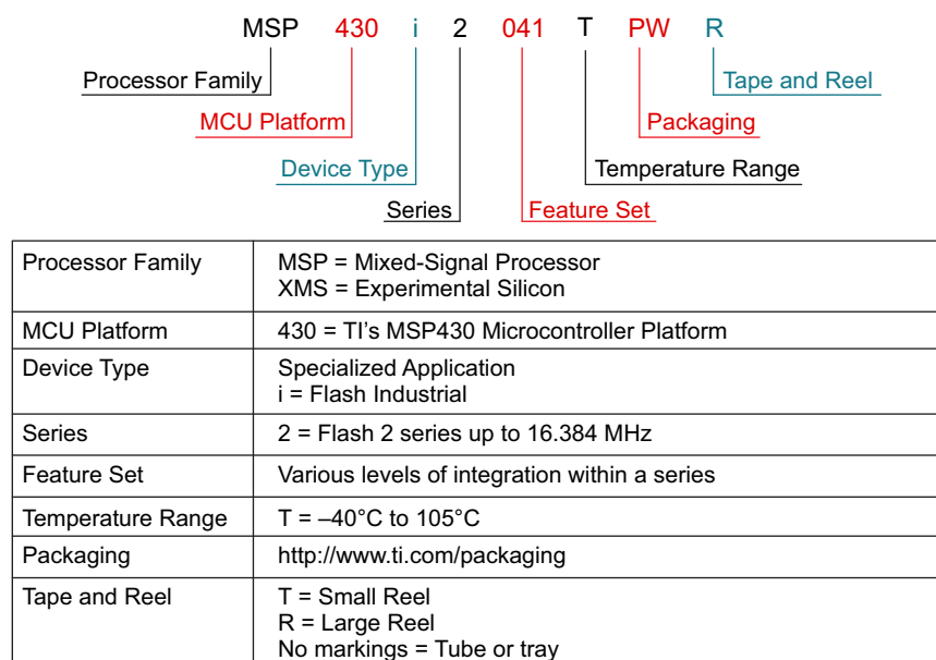
Figure 8-1. Device Nomenclature
