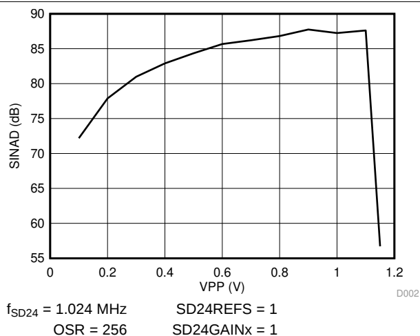
Figure 5-9. SINAD vs VPP
