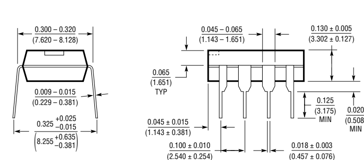
N8 Package 8-Lead Plastic DIP
