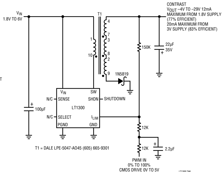
LCD Contrast Supply
