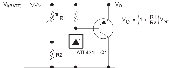
Figure 33. High-Current Shunt Regulator
