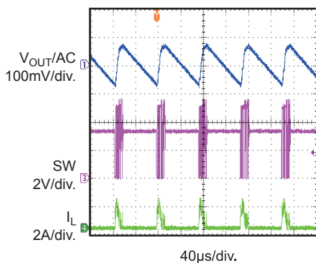
Output-Voltage Ripple Load = 0.1A
