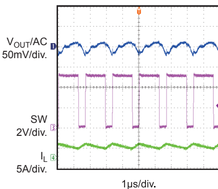
Output-Voltage Ripple Load = 2.1A
