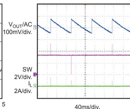
Output-Voltage Ripple Load = 0A
