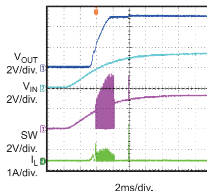
V_IN Startup Load = 0A
