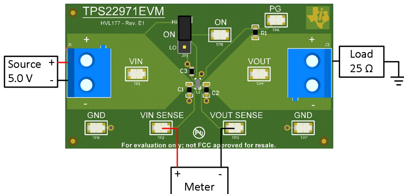
Figure 5. R_{ON} Setup
