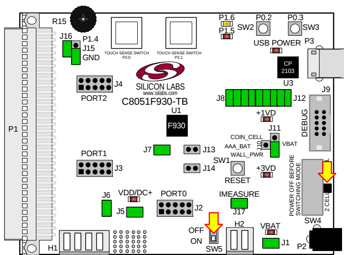
Figure 1. Si1120 Evaluation Board—Shorting Block Settings
