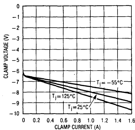
Clamp Voltage
