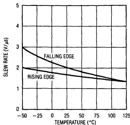
Slew Rate
