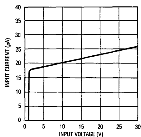
Input Current
