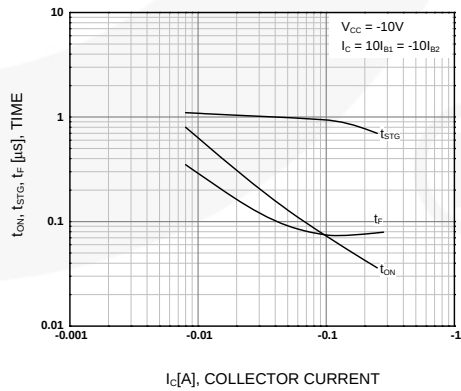
Figure 6. Switching Time
