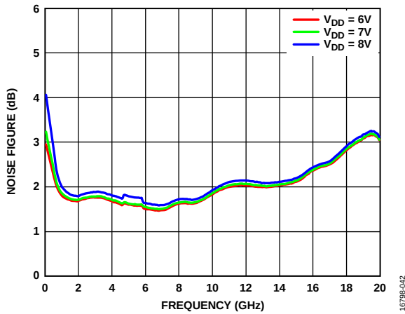
Figure 16. Noise Figure vs. V_{DD}
