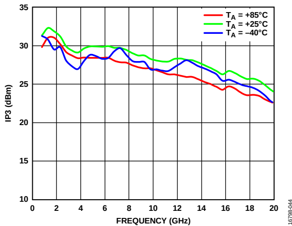
Figure 18. Output IP_3 vs. Temperature
