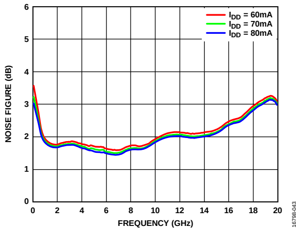
Figure 17. Noise Figure vs. I_{DD}
