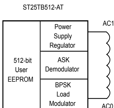
Figure 1. Logic diagram
