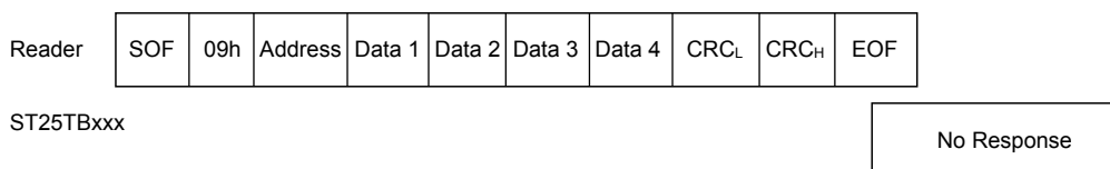
Figure 39. Write_block frame exchange between reader and ST25TB512-AT
