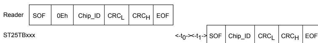
Figure 27. Select frame exchange between reader and ST25TB512-AT
