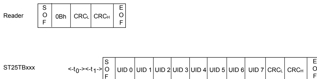
Figure 43. Get_UID frame exchange between reader and ST25TB512-AT
