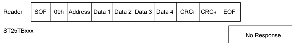
Figure 52. Write_block frame exchange between reader and ST25TB512-AT
