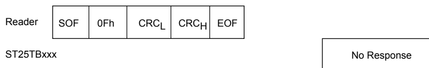
Figure 30. Completion frame exchange between reader and ST25TB512-AT
