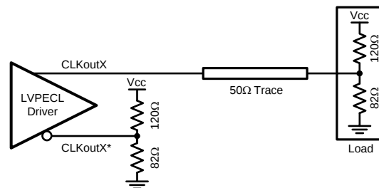
Figure 8-9. Single-Ended LVPECL Operation, DC Coupling
