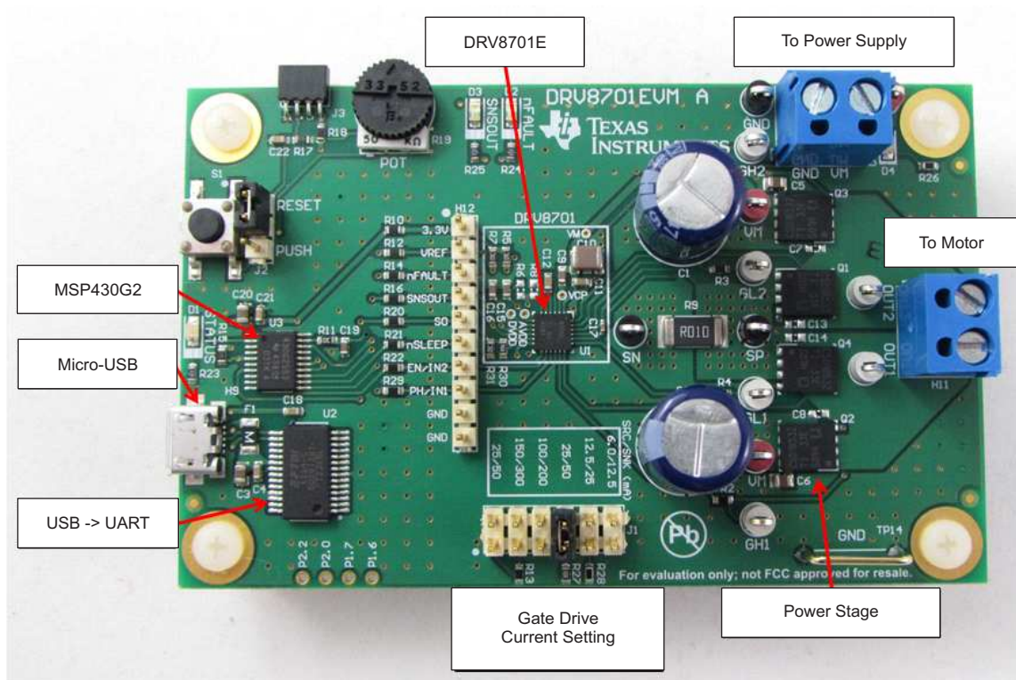
Figure 1. Board Components
