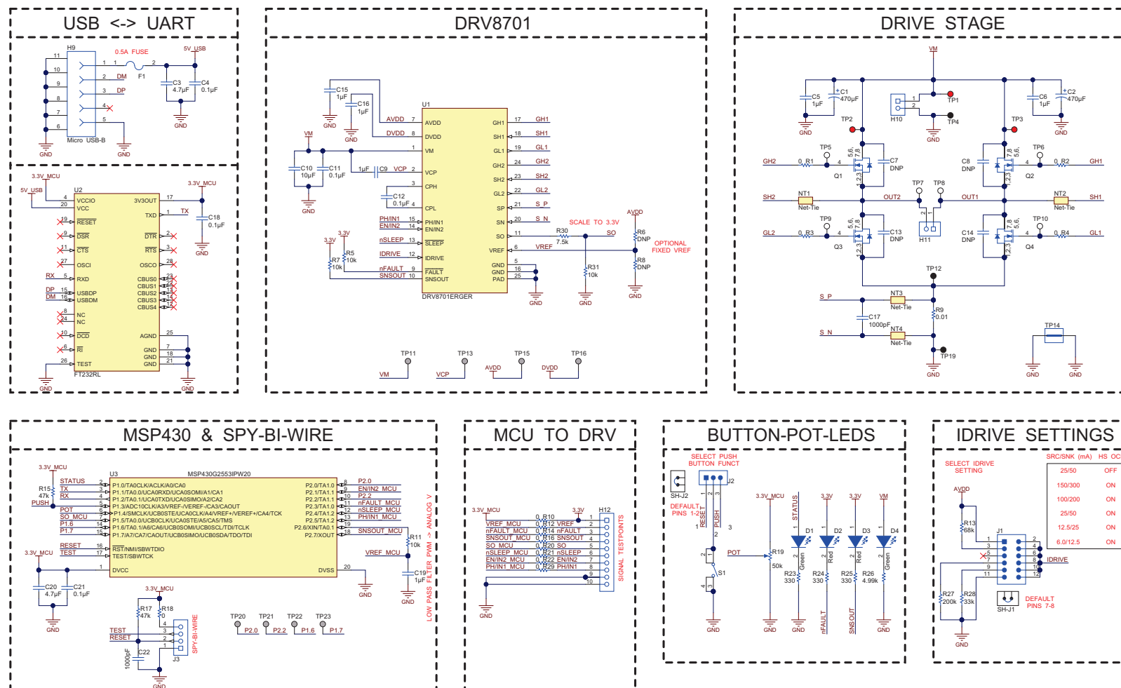
Figure 8. DRV8701EVM Schematic
