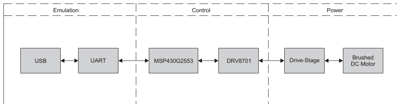
Figure 2. Block Diagram
