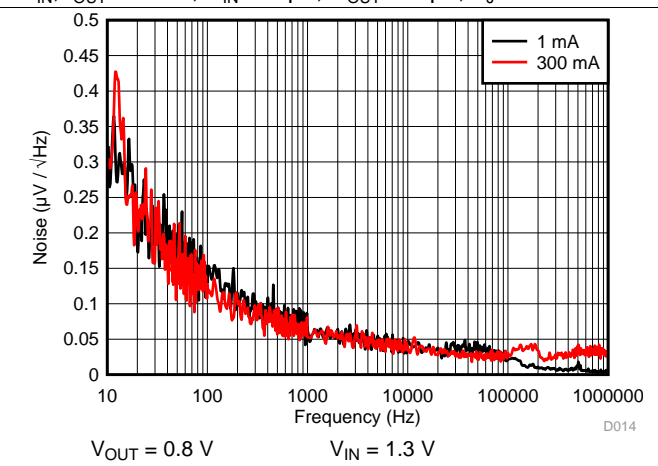
Figure 14. Noise Density
