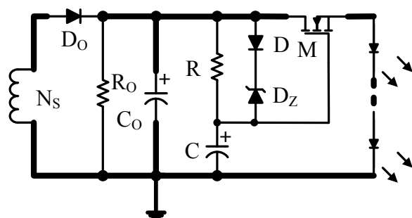
Figure14: Ripple Suppressor
