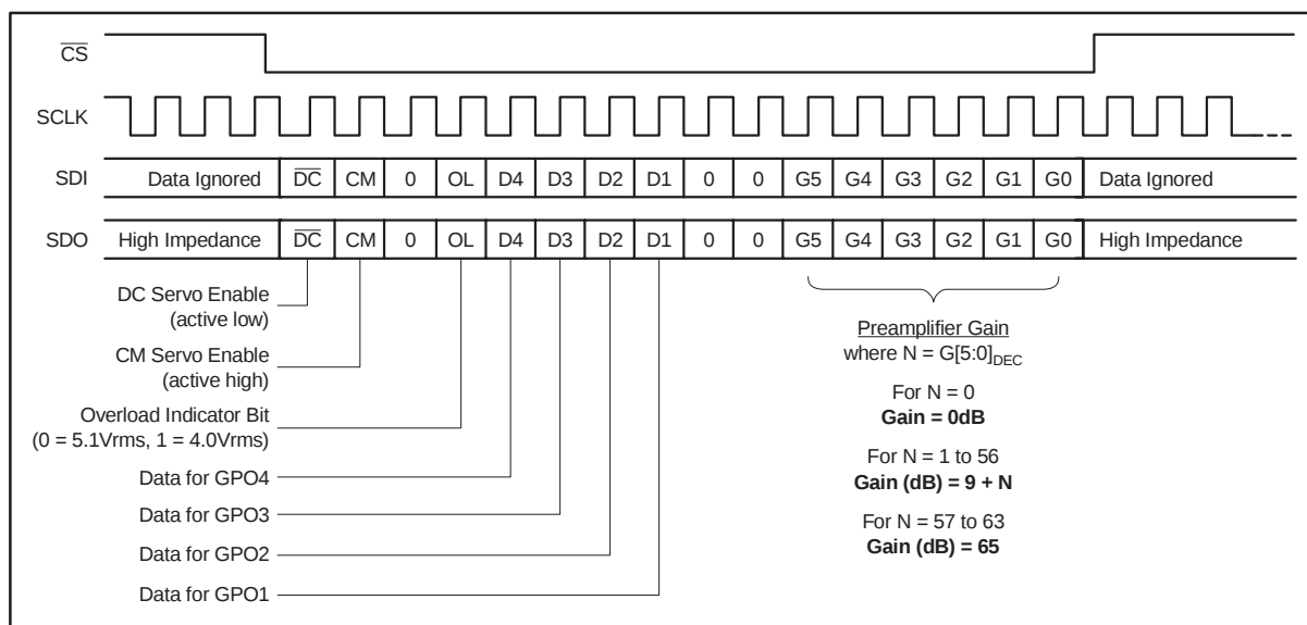
Figure 1–2. PGA2500 Serial Port Protocol
