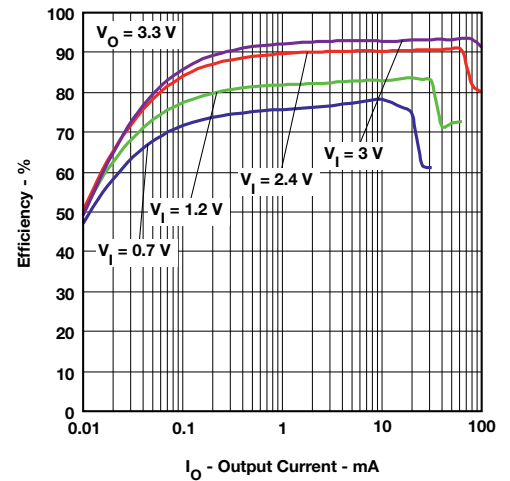
Efficiency versus output current and input voltage.
