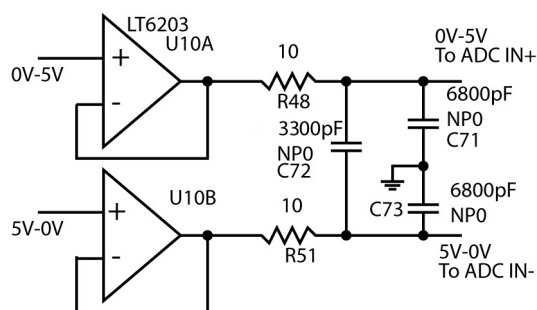
Figure 2. Fully-Differential Driver
