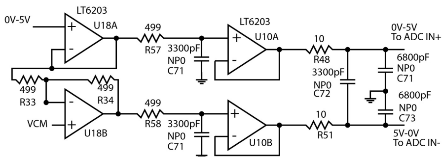
Figure 3. Single-Ended-to-Differential Driver
