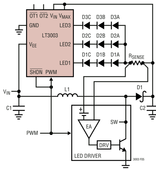
Figure 5. Buck-Boost Mode
