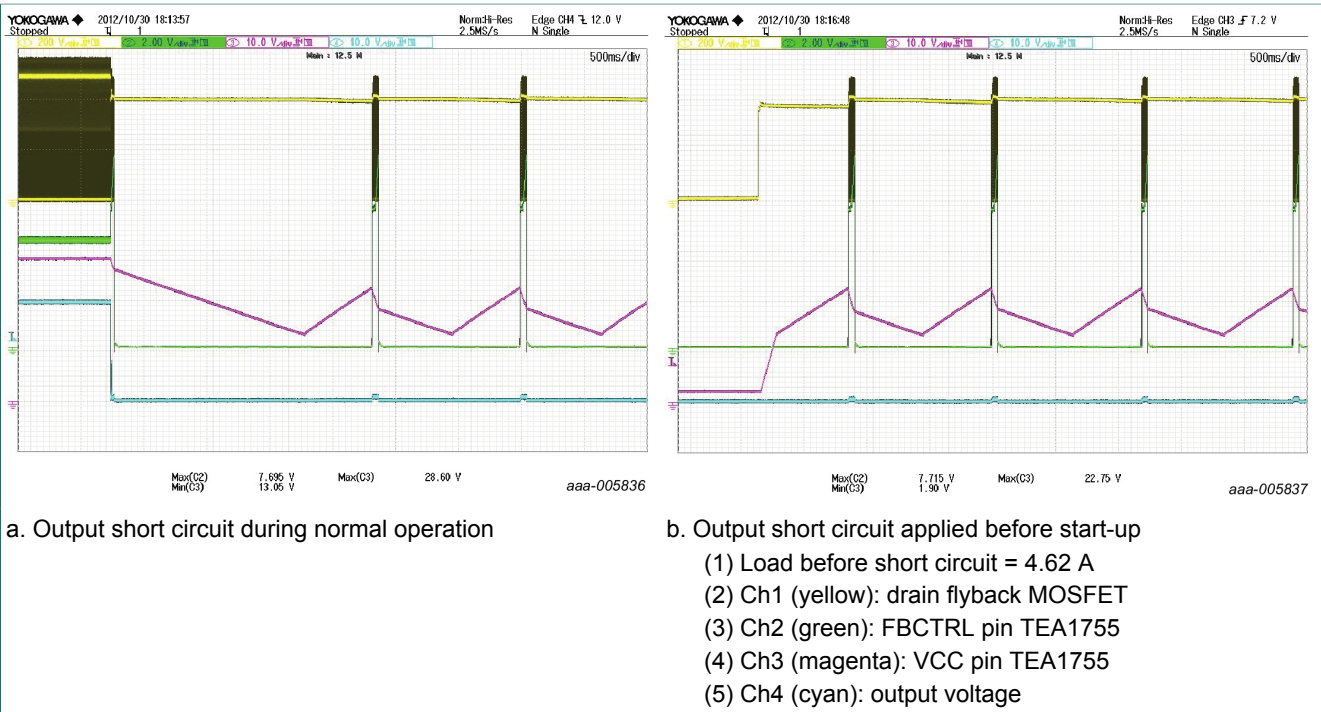
Figure 10. Output short circuit 264 V/50 Hz
