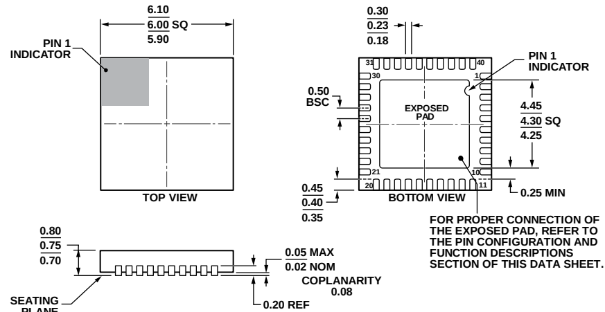
Figure 40. 40-Lead Lead Free Chip Scale Package [LFCSP_WQ] 6 mm × 6 mm Body, Very Very Thin Quad (CP-40-10)
