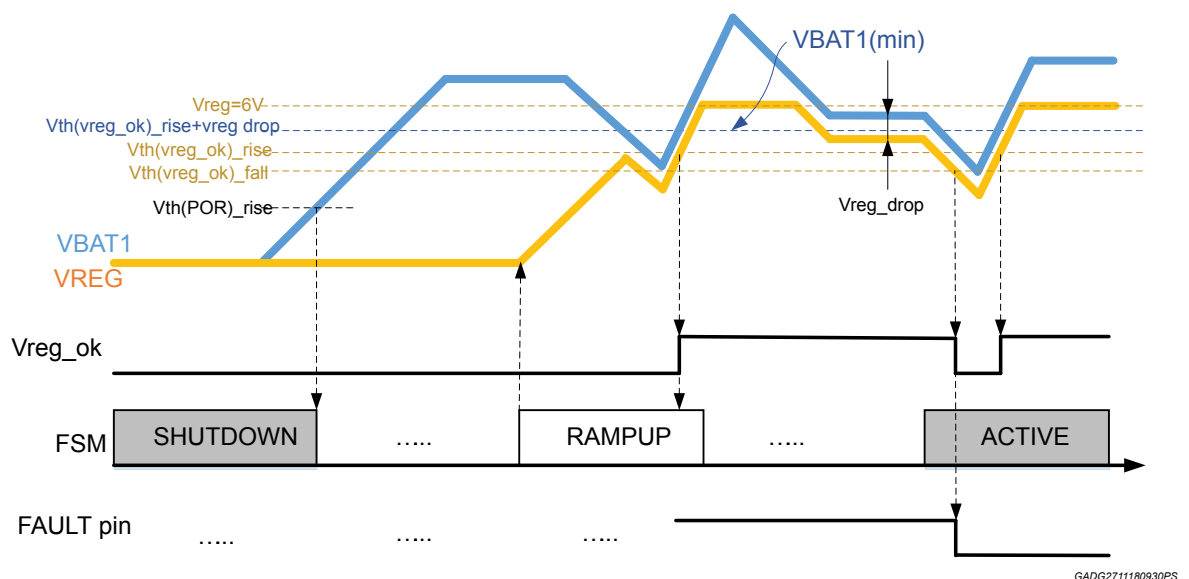
Figure 8. VREG influence on PMIC behavior
