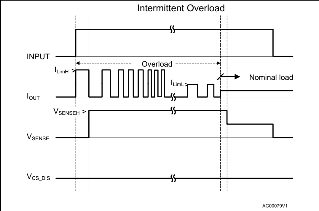
Figure 13. Intermittent overload
