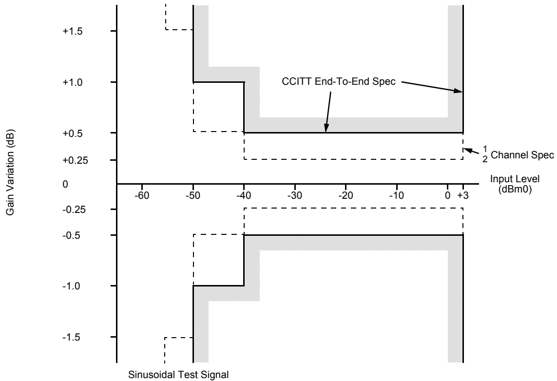
Figure 12 - Variation of Gain With Input Level
