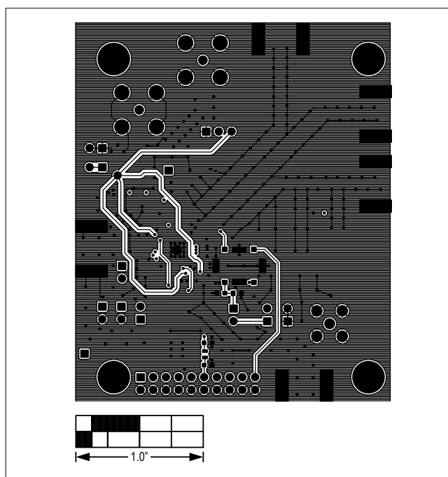
Figure 7. MAX2150 EV Kit Secondary Side
