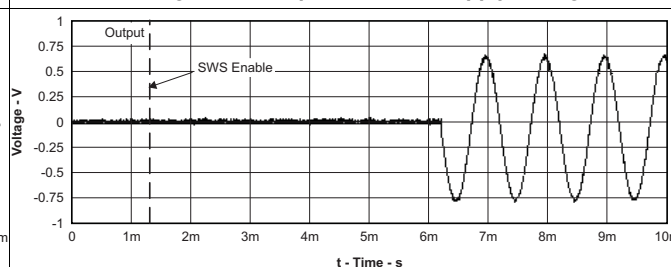
Figure 24. Start-Up Time
