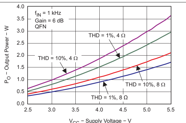
Figure 22. Output Power vs Supply Voltage
