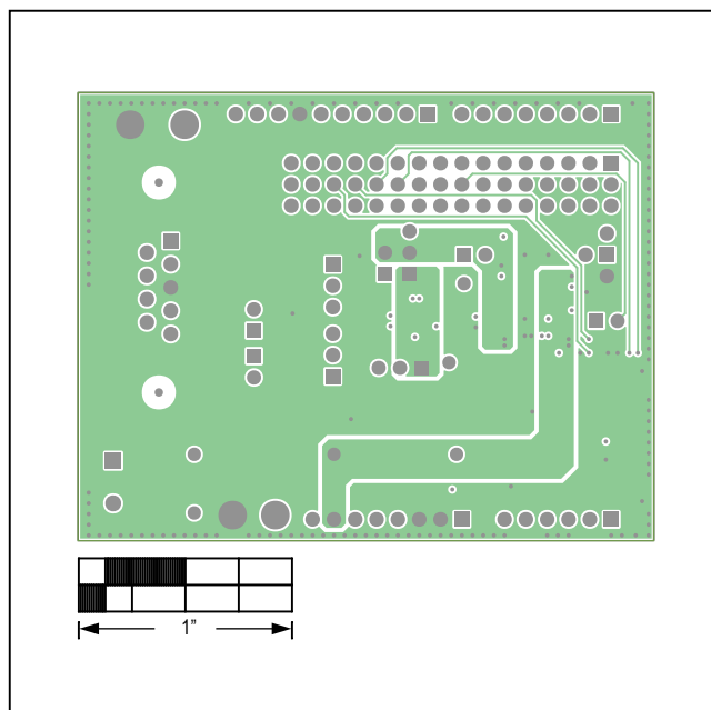
MAX33054E Shield—Internal 3
