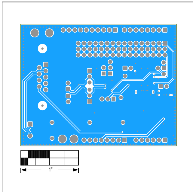
MAX33054E Shield—Bottom
