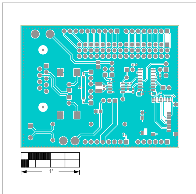
MAX33054E Shield—Top
