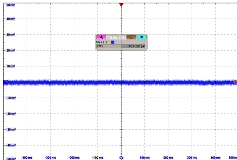
Figure 6. 20mA Loop Current Noise During Silence over 500Ω Load Resistor
