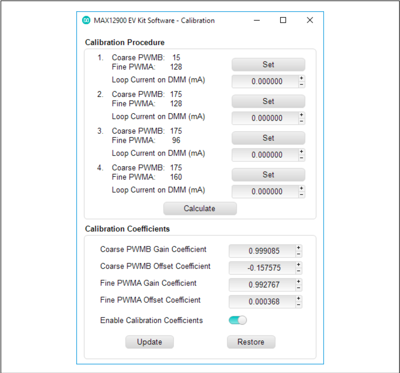
Figure 3. Calibration Window
