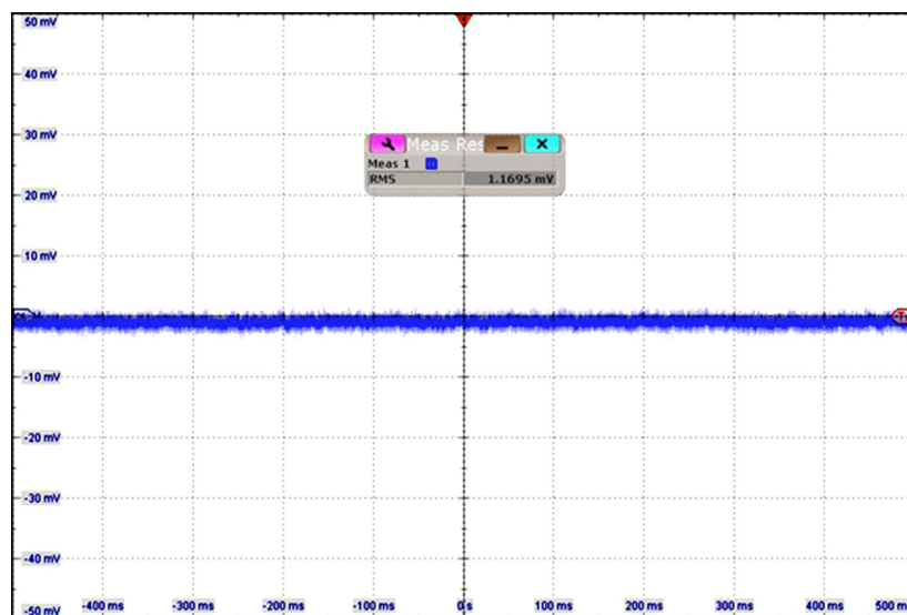
Figure 5. 4mA Loop Current Noise During Silence Over 500Ω Load Resistor
