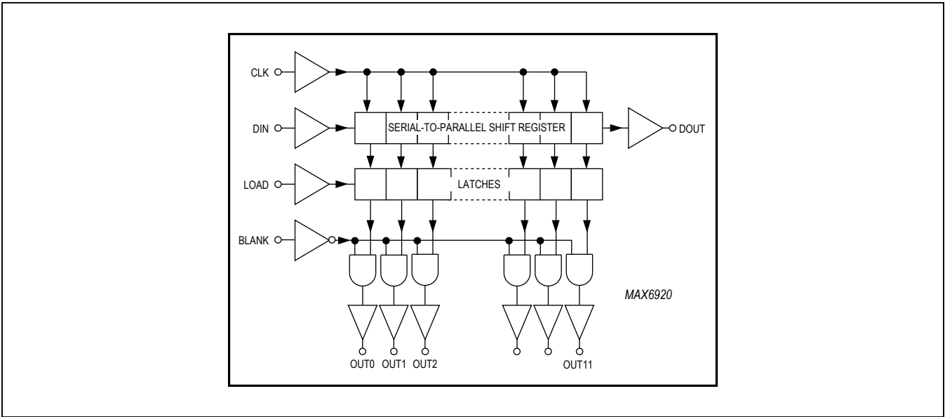
Figure 1. MAX6920 Functional Diagram
