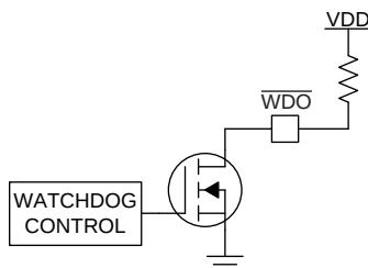
Figure 12. \overline{\text{WDO}} Open-Drain Configuration
