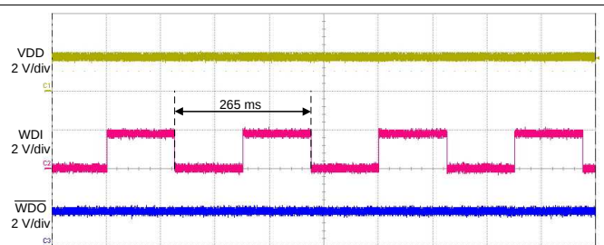
Figure 17. Typical WDI Signal
