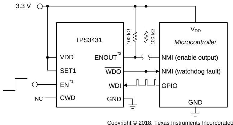
Figure 11. Monitoring a Microcontroller with Standard Watchdog Timer
