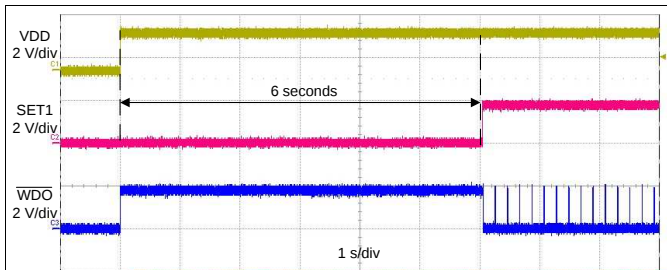
Figure 16. Startup Without a WDI Signal
