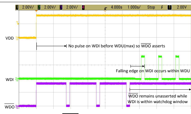
Figure 14. \overline{WDO} Fault Caused by missing WDI Pulses Followed by Correct Timing WDI Pulses
