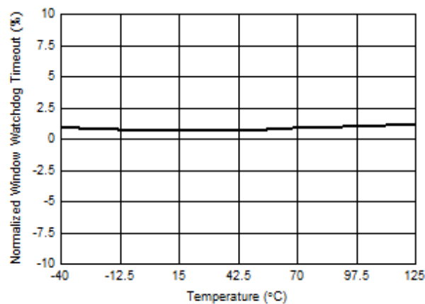
Figure 7. Normalized Watchdog Timeout ( t_{WD} ) Accuracy (SET1 = 1, CWD = 10kΩ)
