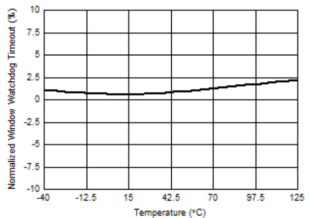
Figure 6. Normalized Watchdog Timeout ( t_{WD} ) Accuracy (SET1 = 1, CWD = NC)
