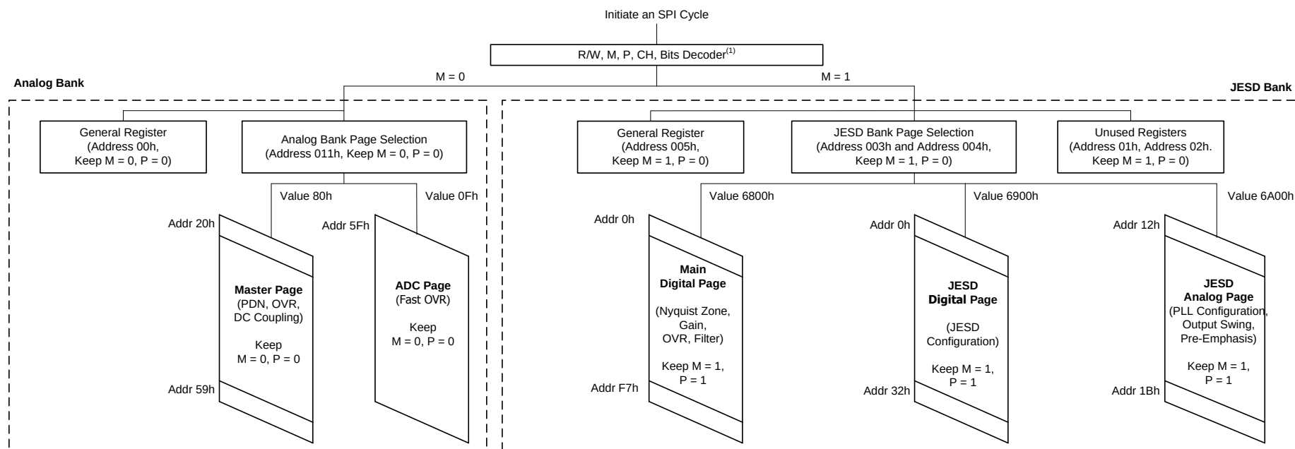
Figure 80. Serial Interface Registers
