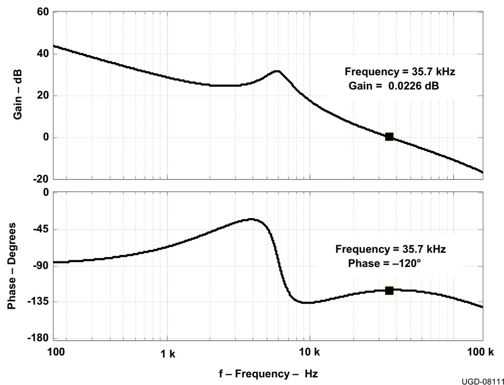
Figure 11. Bode Plot of the Design Example Circuit by Simulation ( V_{IN}=12 V and I_{OUT}=0 A)
