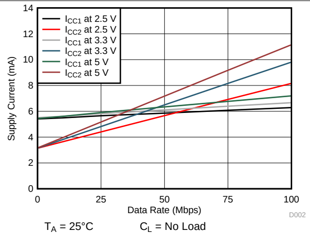
Figure 6. ISO7760-Q1 Supply Current vs Data Rate (With No Load)
