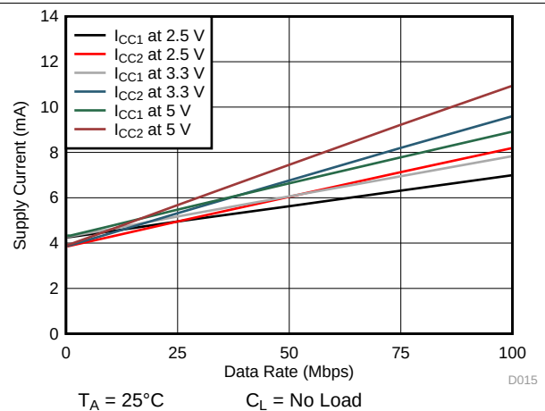
Figure 10. ISO7762-Q1 Supply Current vs Data Rate (With No Load)
