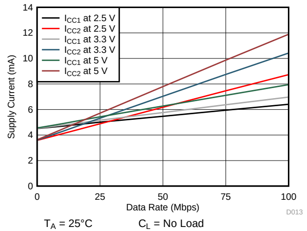
Figure 8. ISO7761-Q1 Supply Current vs Data Rate (With No Load)
